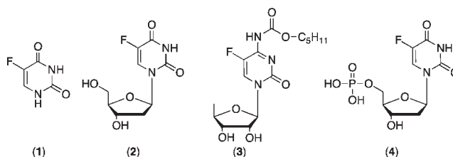
Figure 1. Some fluorinated pyrimidines.
